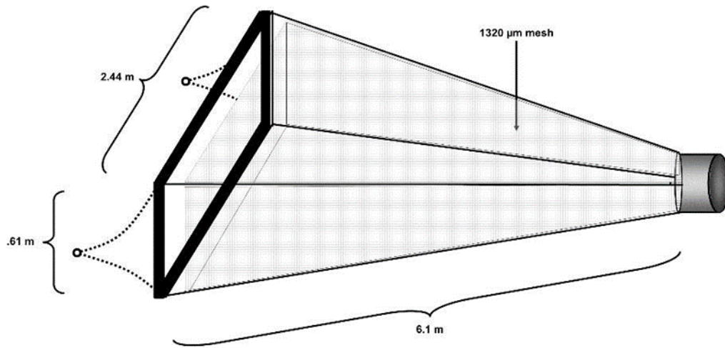
Figure 6. Diagram of the larval sampling net and frame.
